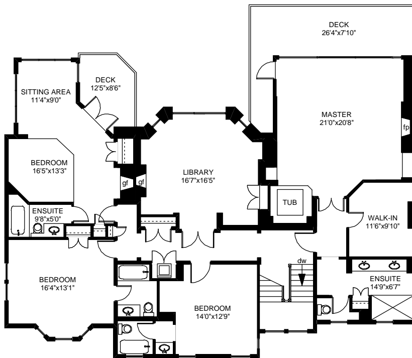
SECOND FLOOR 2544 SQ.FT
